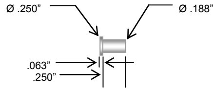
CASE STYLE "B"
